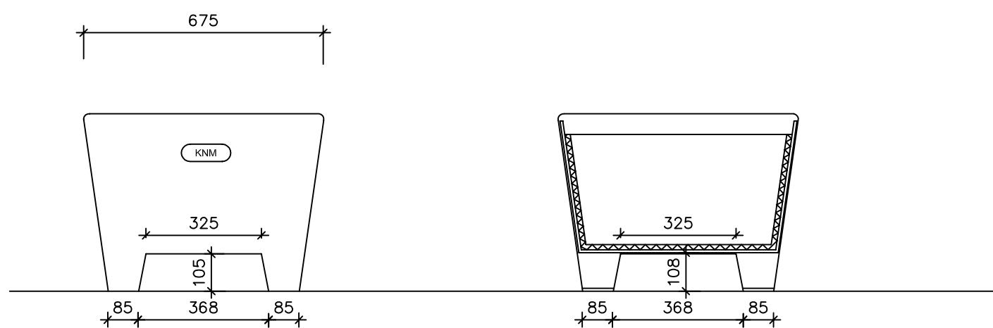
GAVEL - PLANTERINGSKÄRL 2
