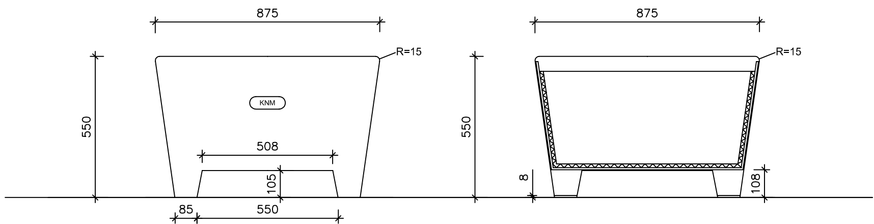
GAVEL - PLANTERINGSKÄRL 1
