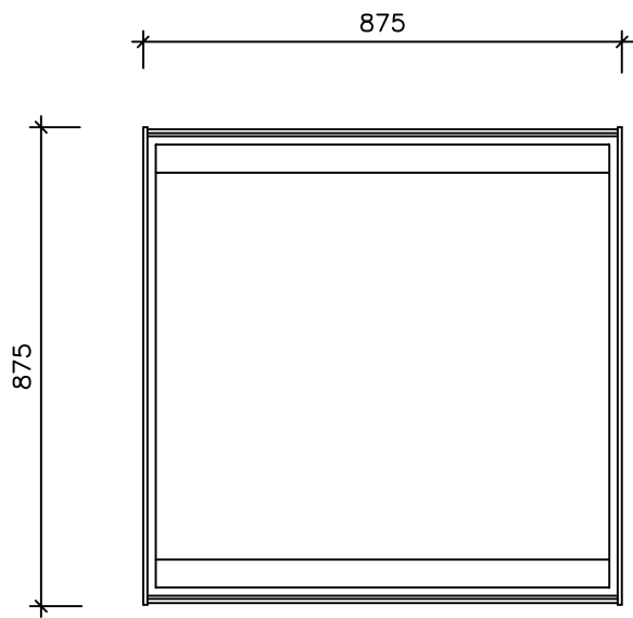
PLAN - PLANTERINGSKÄRL 1
